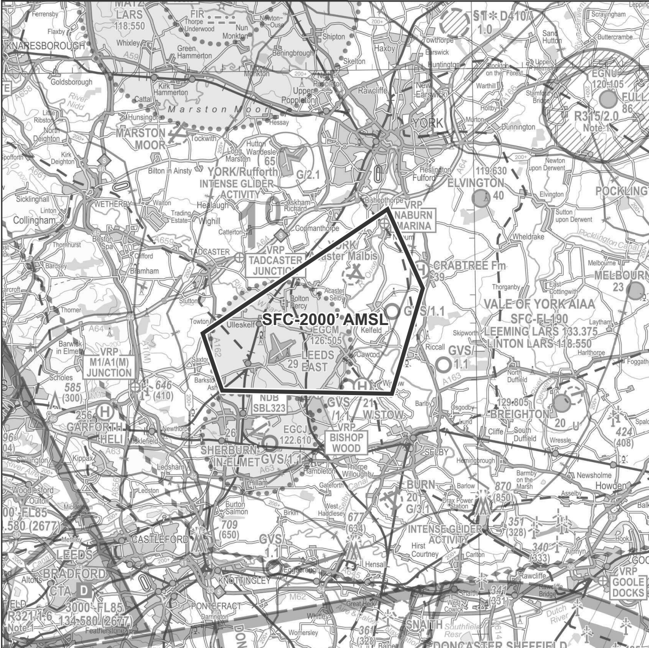
2021_082_Leeds East Aero Race_GRAPHIC DRAWN 06JUL21
